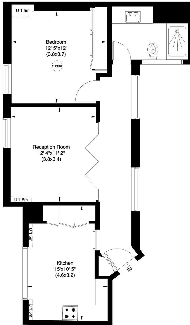
Fifth Floor
